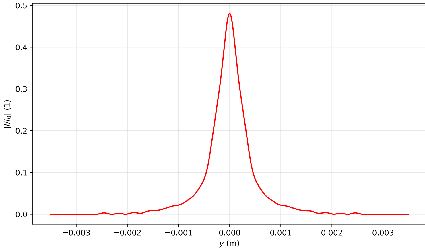
Intensity profile I(x = 0, y, z = 2.229)/I_0 , P_{in}=3.0P_{cr} , artificial time
